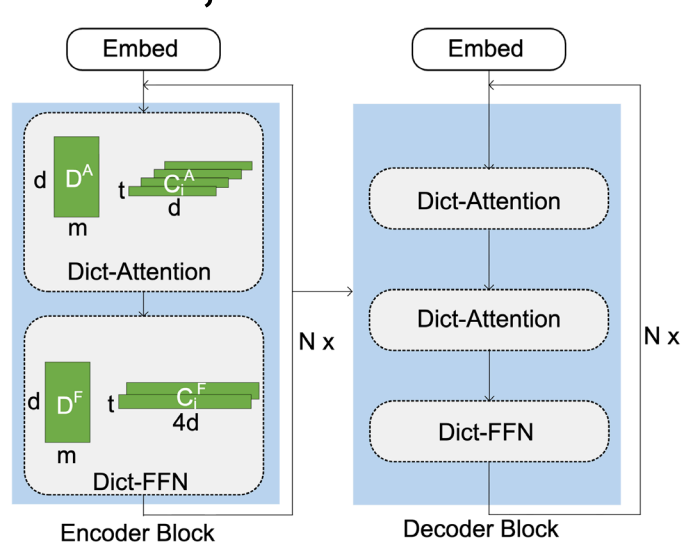
DictFormer [ICLR22]
