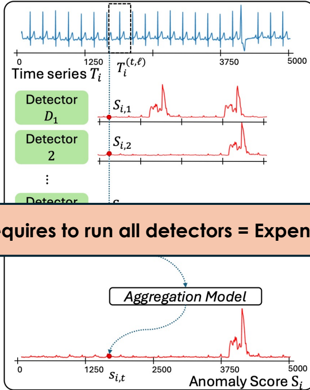
(a) Ensembling
